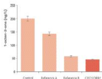
Figure 2: Influence of GEOSORB® (40g/hL) on octenone content found in a white wine.
